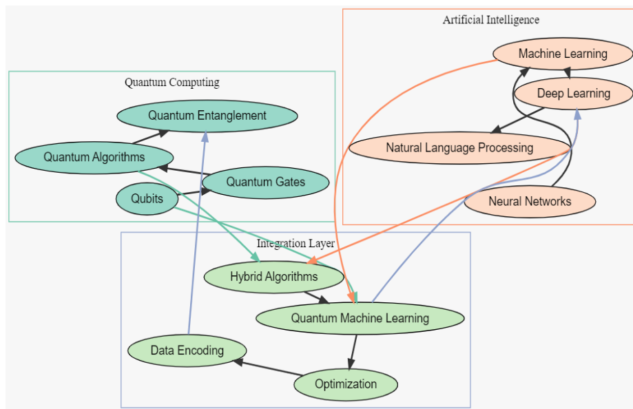
Figure 1: Quantum-AI Integration
