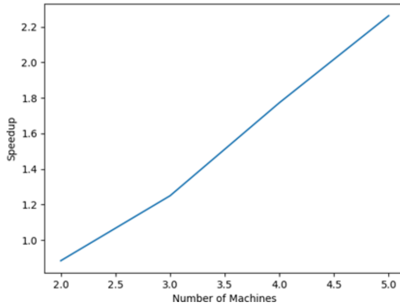
Figure 2: Scalability of DistribuScript
