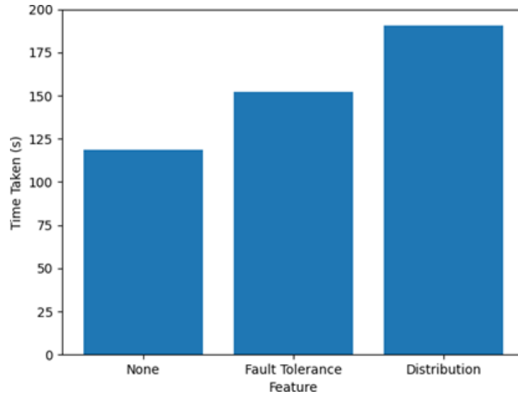
Figure 3: Performance of DistribuScript with Fault Tolerance and Distribution Features
