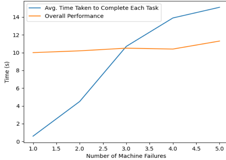
Figure 1: Performance of DistribuScript under Machine Failures
