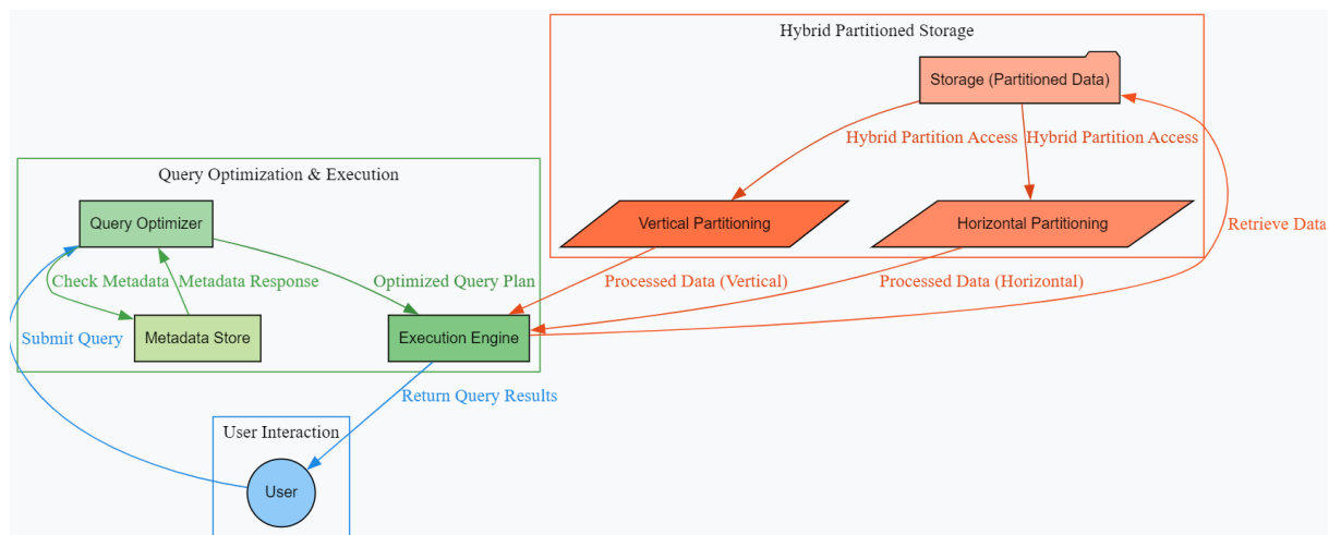
Figure 1: Cloud Data Warehouse Query Optimization and Hybrid Partitioning Architecture
