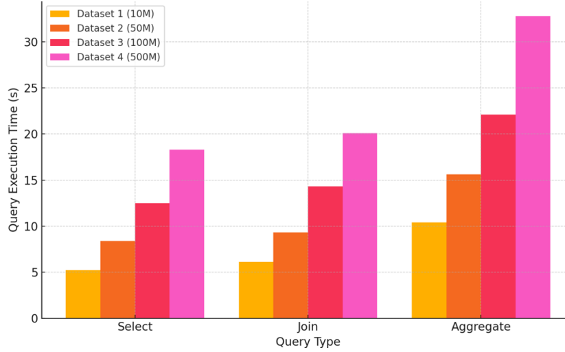
Figure 2: Comparison of the execution time of various partitioning strategies across different query types
