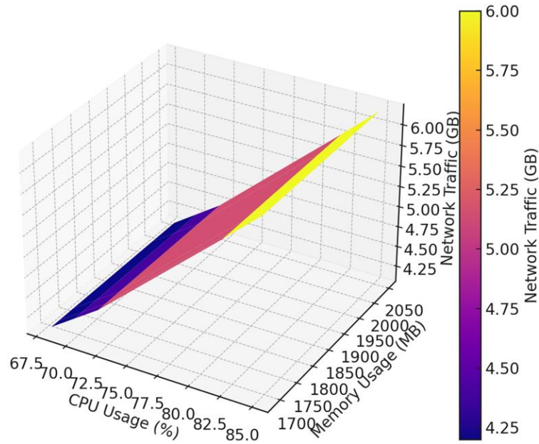
Figure 3: Impact of different partitioning strategies on resource consumption as the query complexity increases
