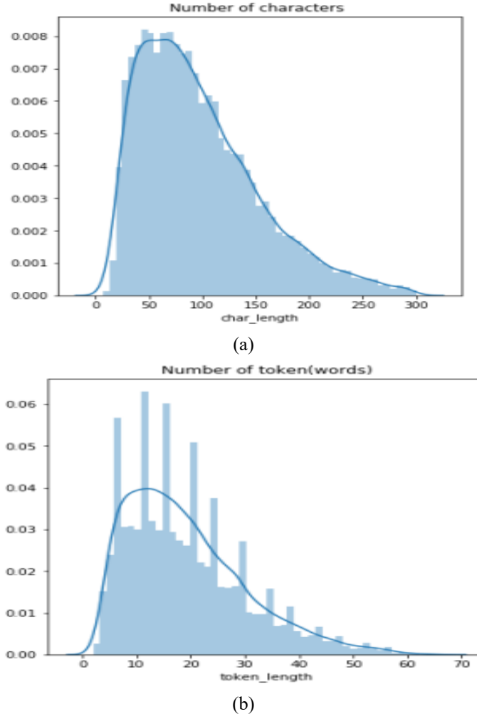
Figure 8: (a) Characters input graph (b) tokenization input graph
