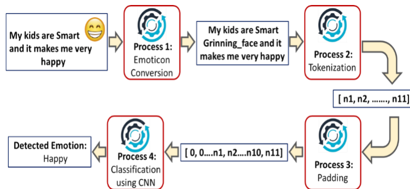
Figure 2: The proposed ER architecture for a sample set of text and emoticon-based microblog data [49]
