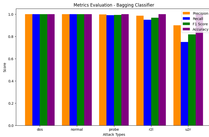
Figure 11: Metrics Evaluation of Bagging Classifier
