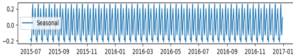
Figure 10: Seasonal component graph
