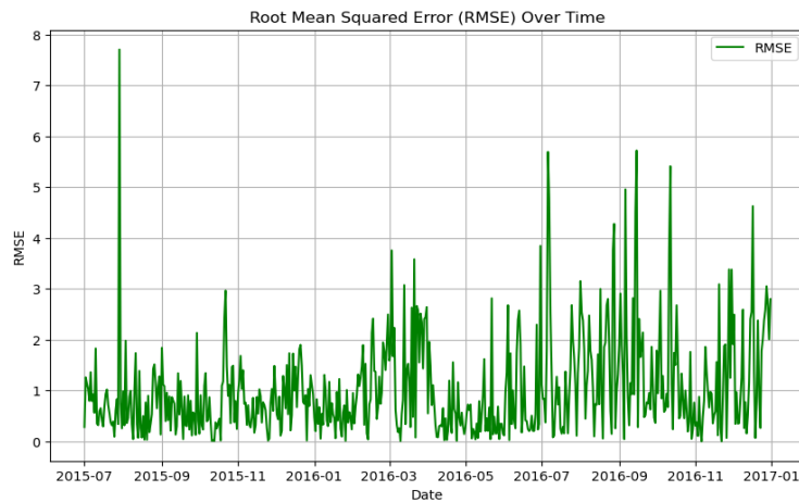
Figure 14: Root mean squared error graph
