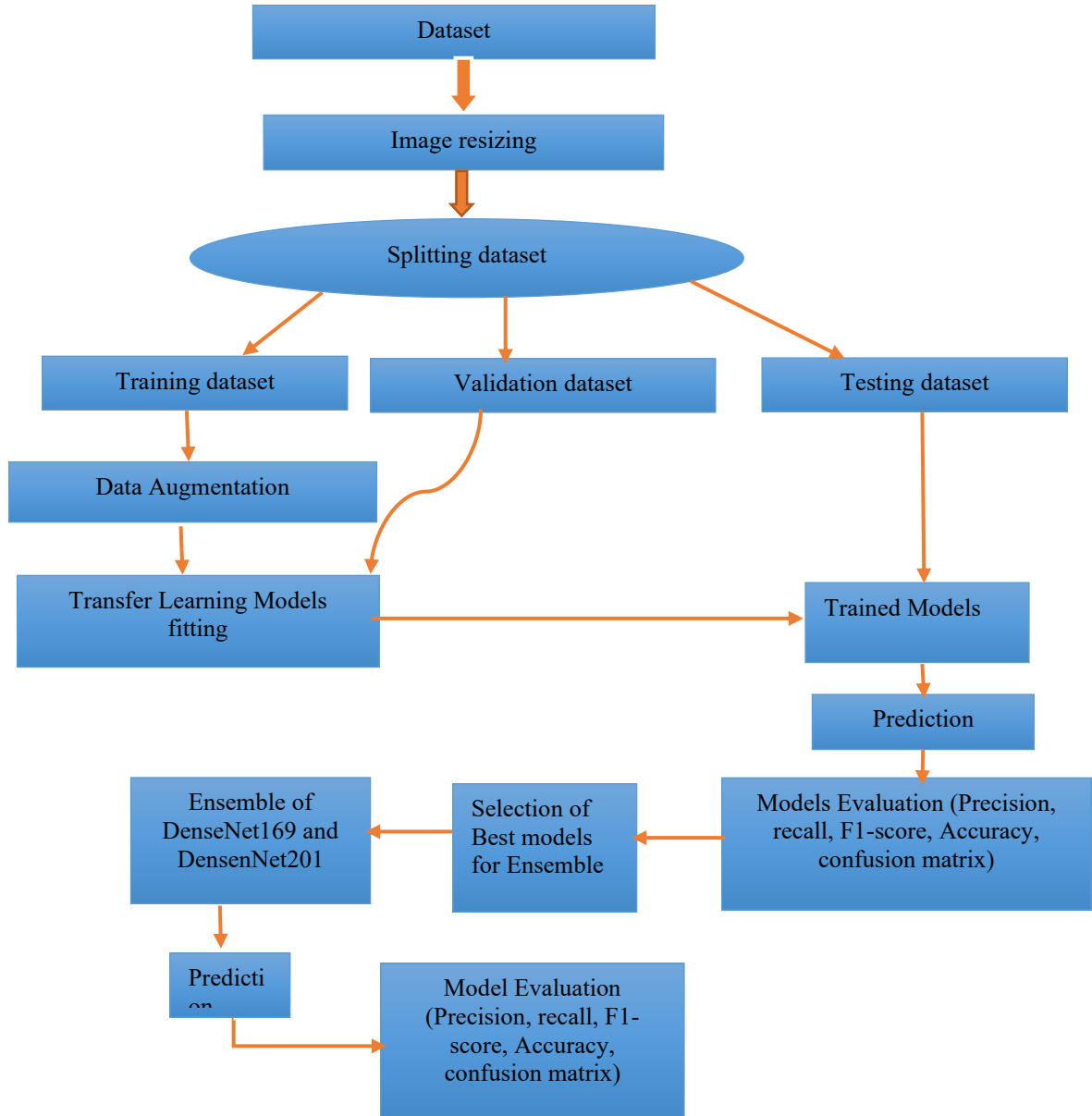
Figure 3: Proposed Methodology
