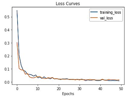
(c) DenseNet121
