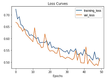
(f) ResNet50
