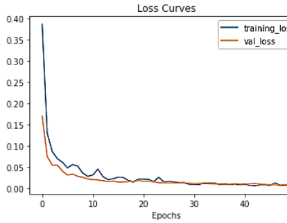
(b) DenseNet201
