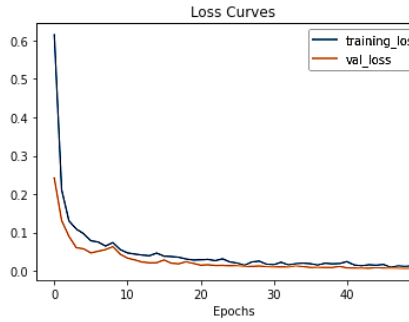
(a) DenseNet169
