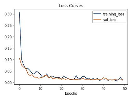
(i) MobileNetV2
