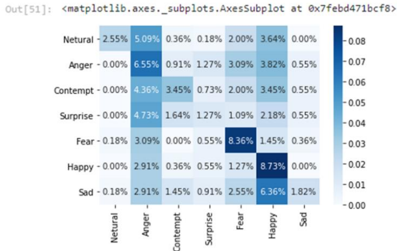
Figure 8: Confusion matrix for facial expressions with micro expressions like neutral, anger, contempt, surprise, fear, happy, and sad
