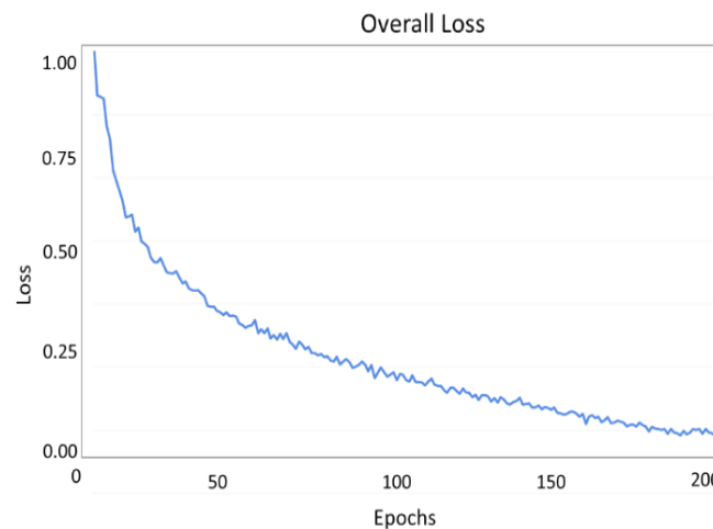
Figure 6: Loss curve of YOLOv8
