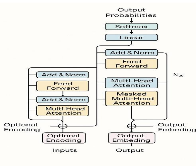
Figure 3: Model architecture
