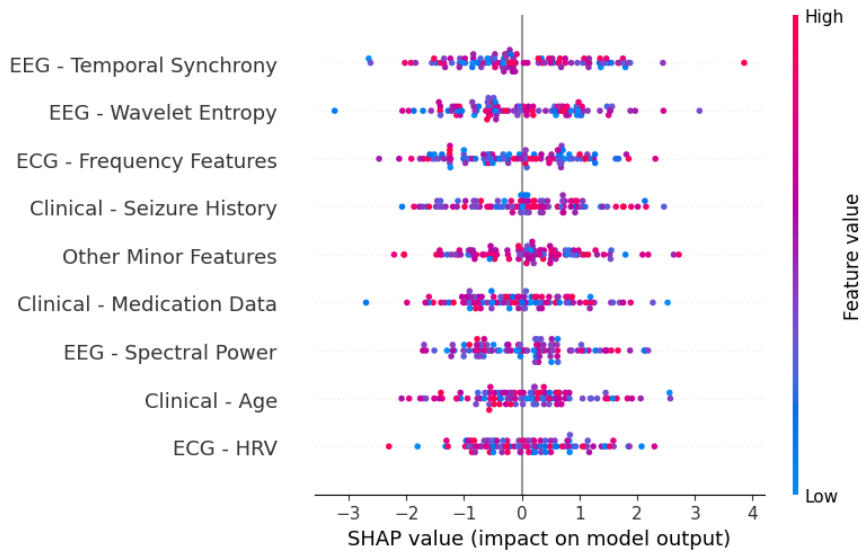
Figure 6: SHAP explainability
