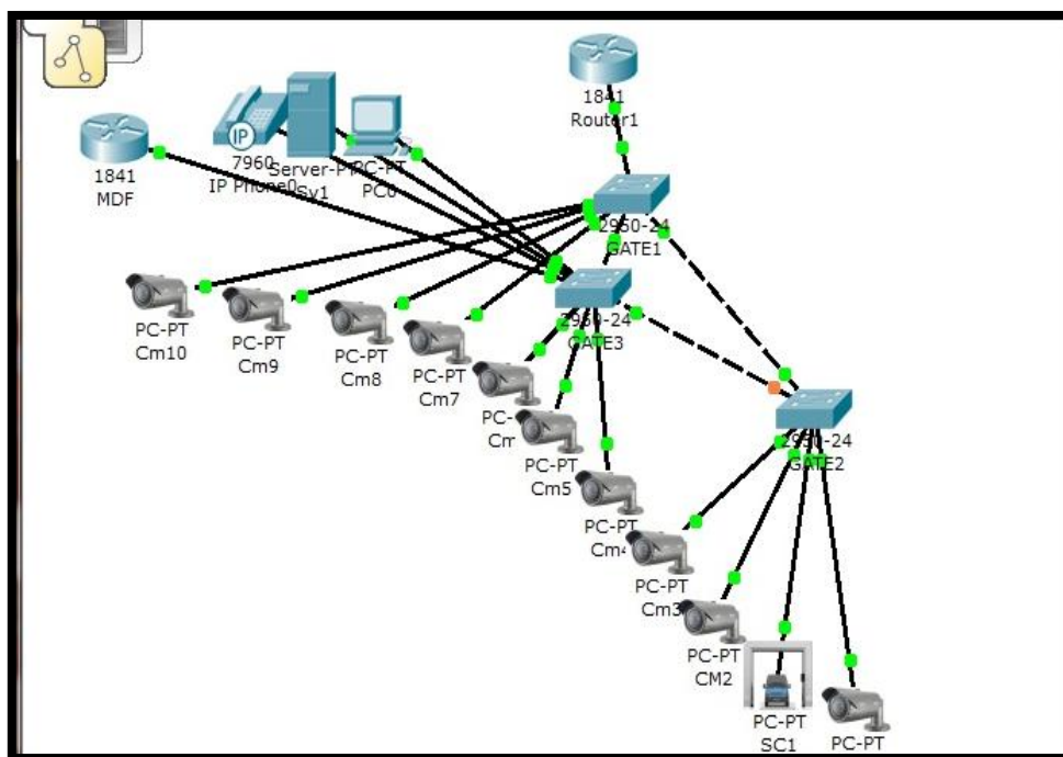
Figure 4: Gate Network Using Packet Tracer Simulator
