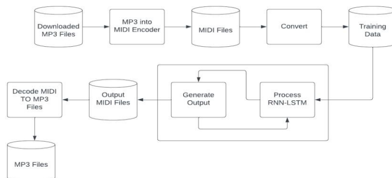
Figure 1: Architecture Diagram
