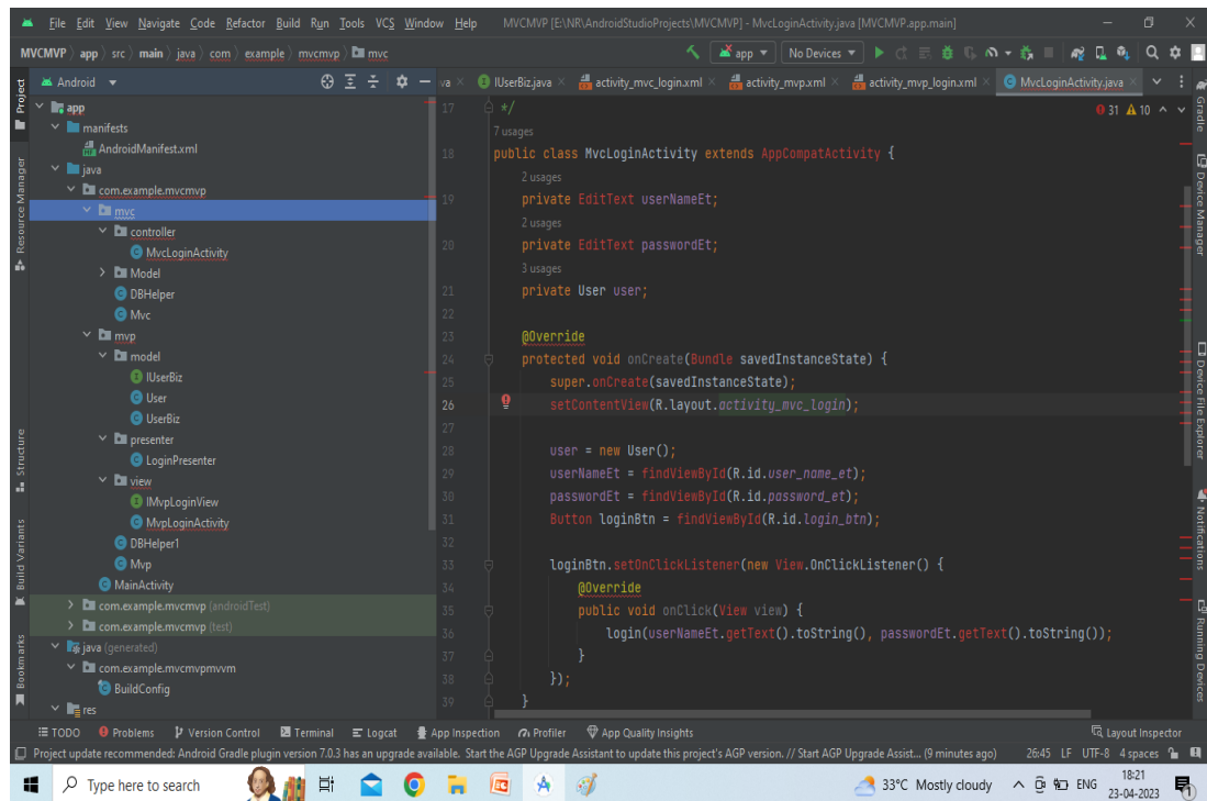
Figure 7: MVC Implementation in Android
