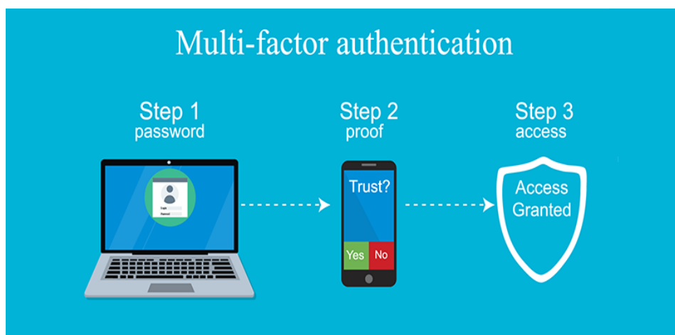
Figure 4: Multi-factor authentication [11]
