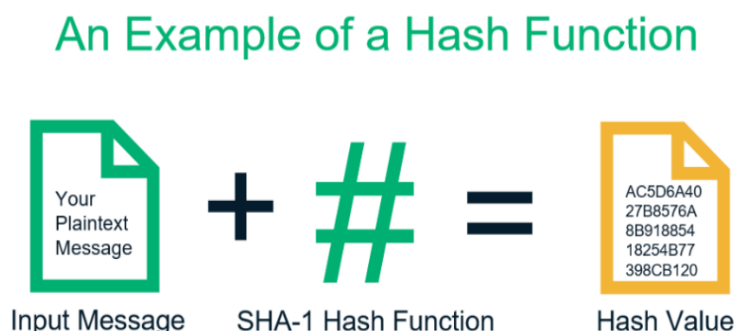
Figure 2: Hash functions [10]
