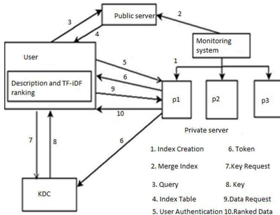
Figure 2: System Architecture
