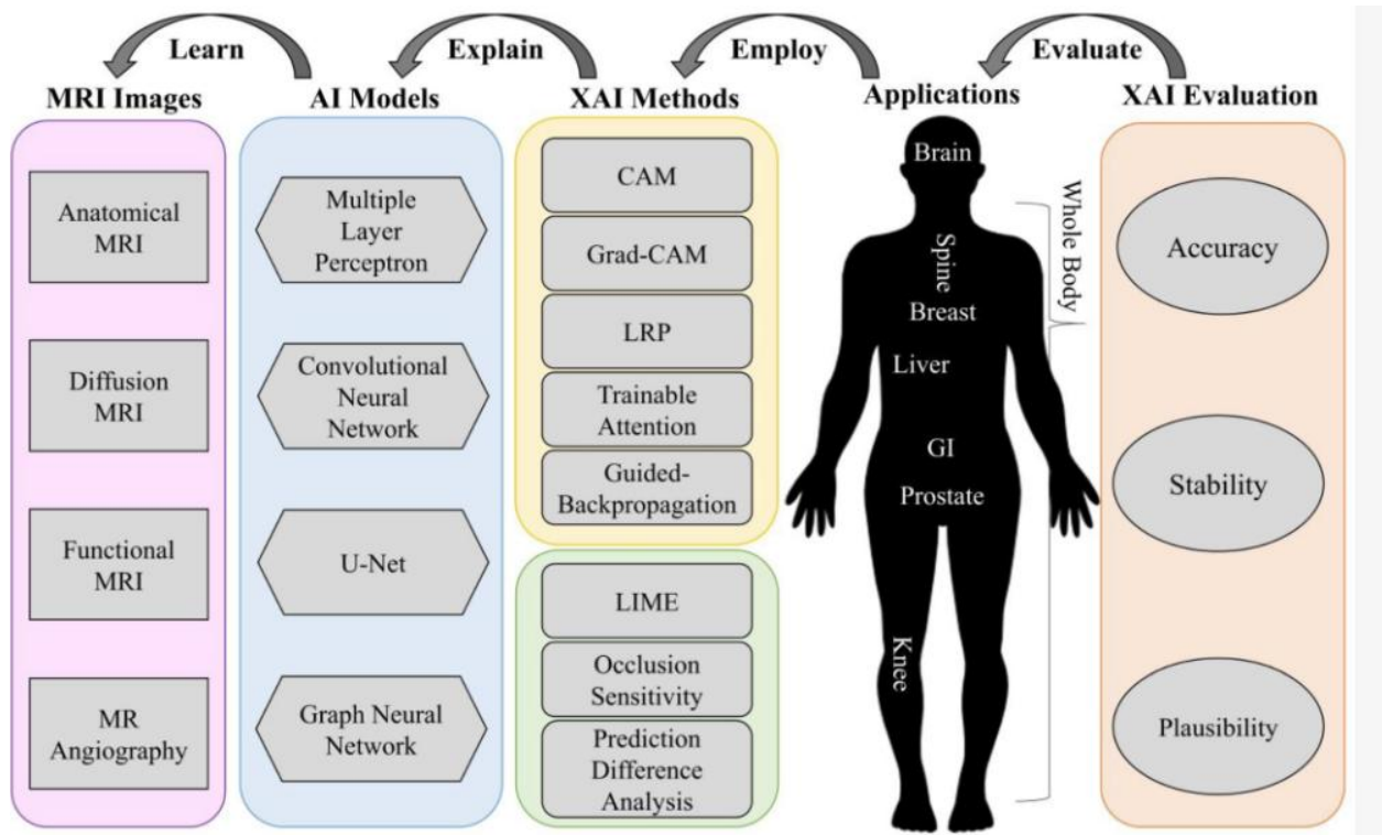
Figure 1: Knowledge Graphs [28]
