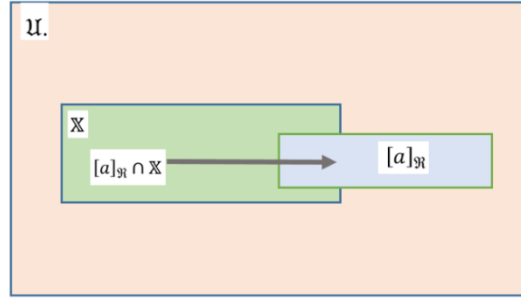
Figure 1: Rough Membership Function
