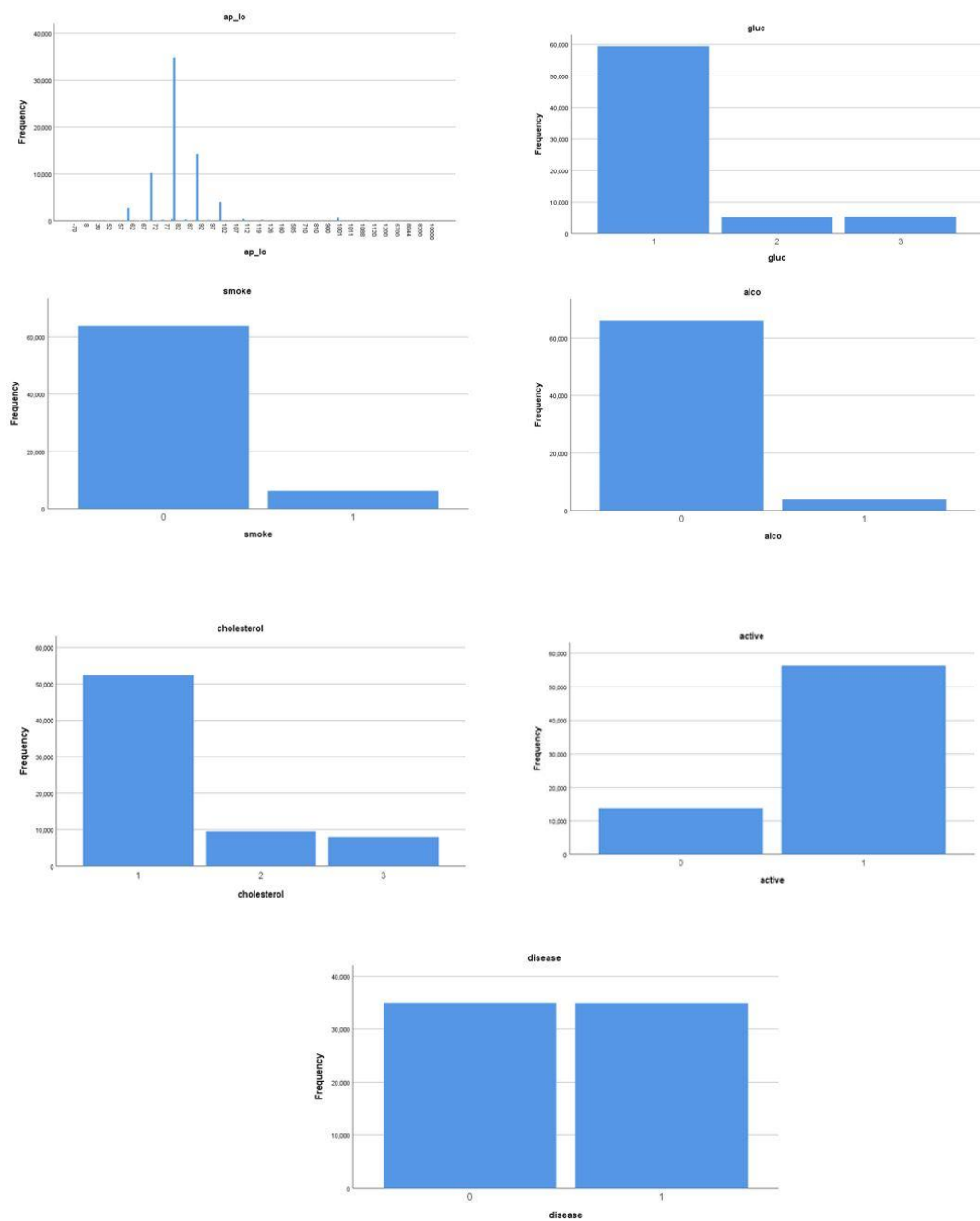
Figure 2: Descriptive statistics
