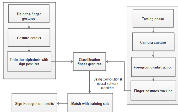
Figure 1: Architectural Diagram of Proposed Methodology
