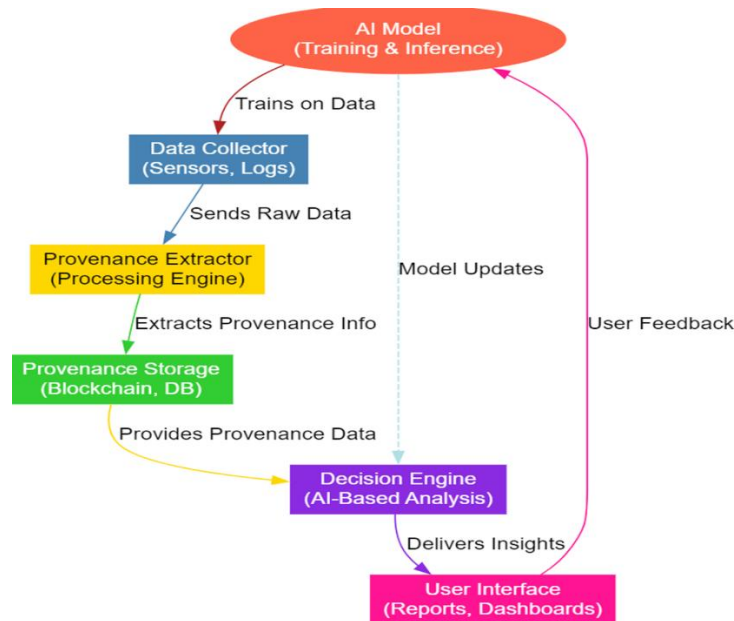
Figure 1: AI-driven data provenance architecture
