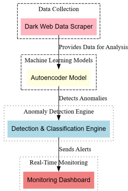
Figure 1: Dark web activities anomaly detection system architecture
