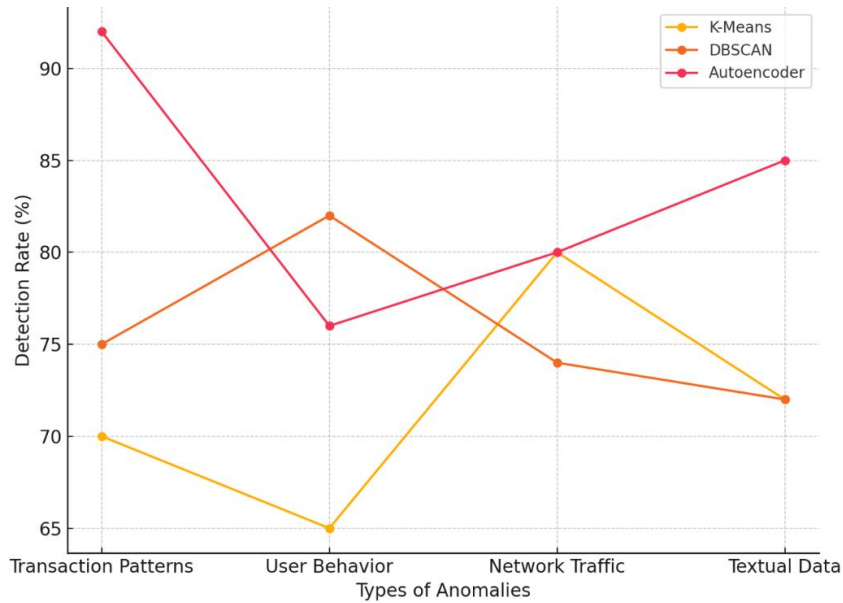
Figure 3: Multi-line graph representing detection rates for varying anomaly types
