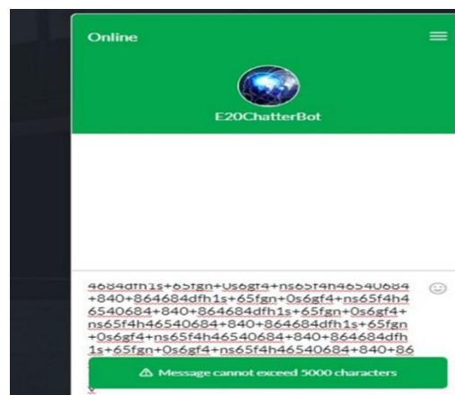
Figure 46: Stress testing
