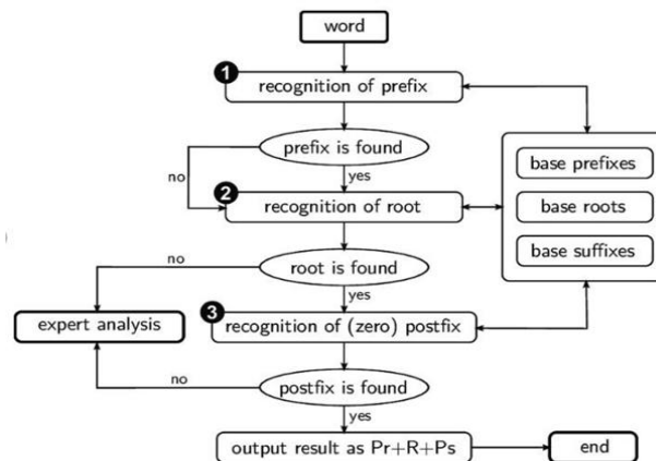
Figure 5: Morphological flow
