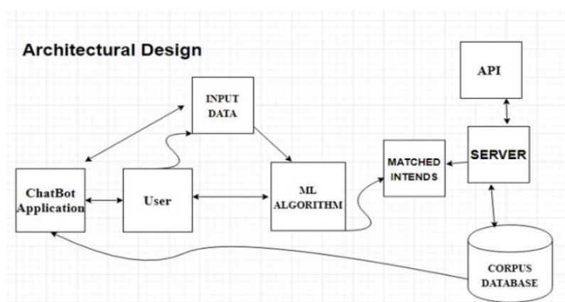
Figure 25: Architectural design
