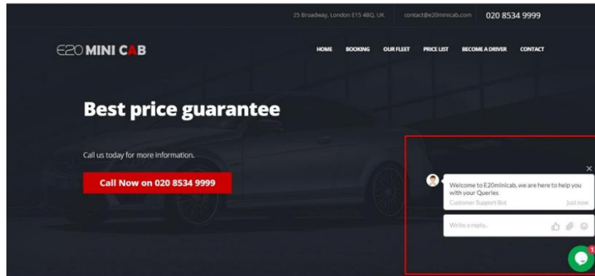
Figure 39: Chatbot appears
