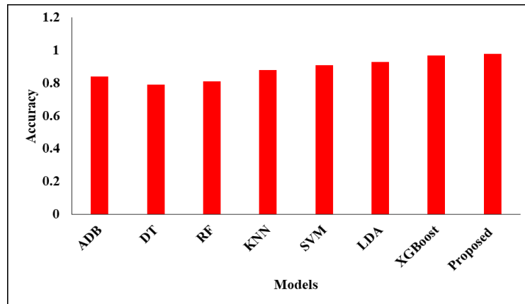
Figure 5: Accuracy analysis
