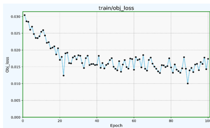
Figure 5: Object loss in skin cancer detection
