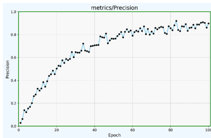
Figure 7: Precision over the epoch of skin cancer detection
