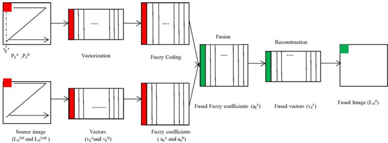
Figure 7: Fuzzy representation
