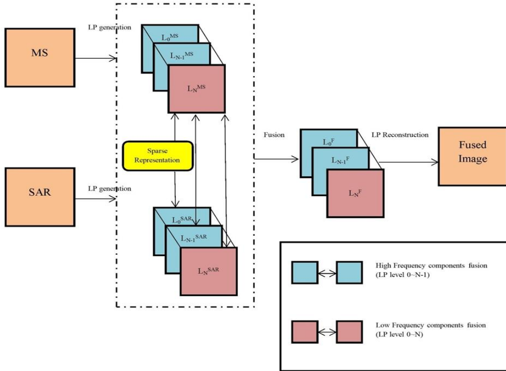
Figure 8: Sparse representation
