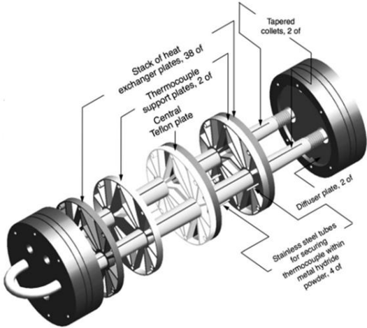
Figure 2: Three-dimensional depiction of heat exchanger assembly [14]
