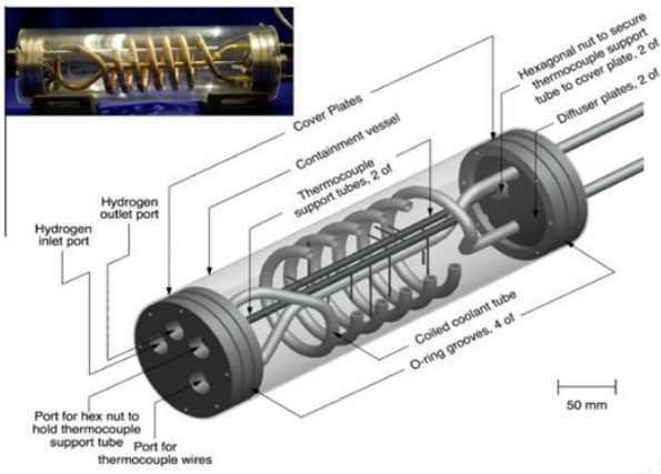
Figure 3: 3-D illustration of containment vessel/heat exchanger assembly [16]
