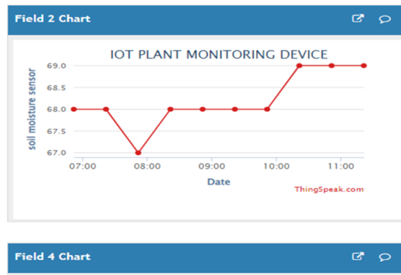
Figure 5: Soil moisture sensor monitoring in the IoT platform
