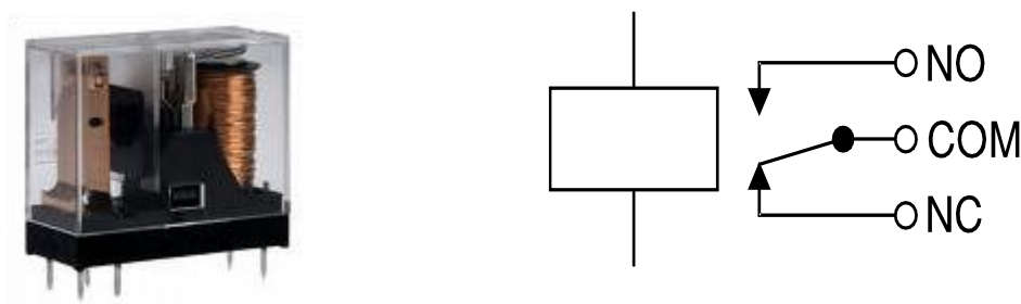
Figure 2: Picture and schematic representation of a relay [8]
