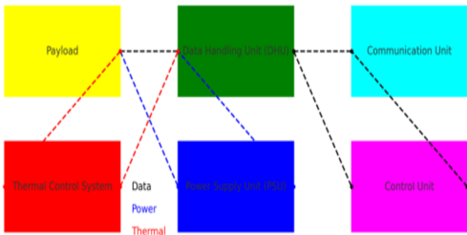
Figure 1: Simplified Electrical Architecture of a Generic Payload System
