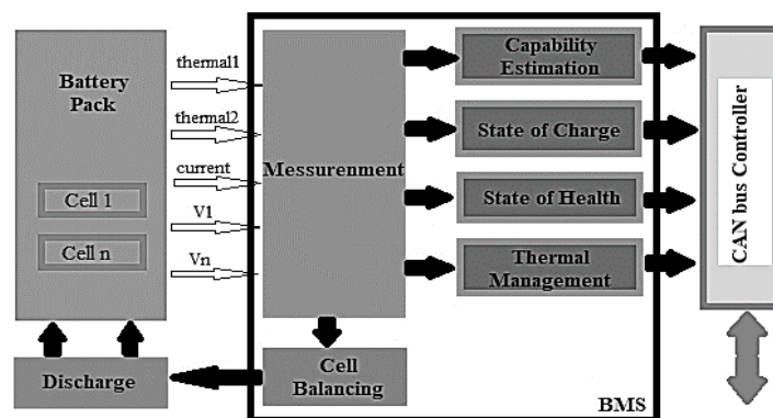
Figure 1: Block diagram of BMS
