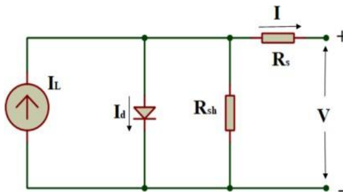
Figure 3: Equivalent Circuit of Solar cell
