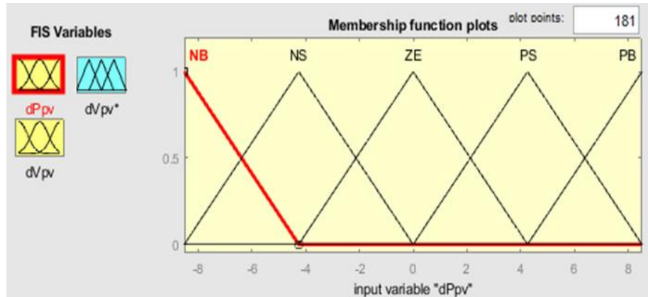
Figure 9: Membership function of the first input variable ( \Delta PPV )
