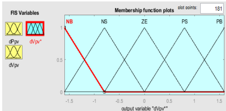
Figure 11: Membership function for duty cycle ratio
