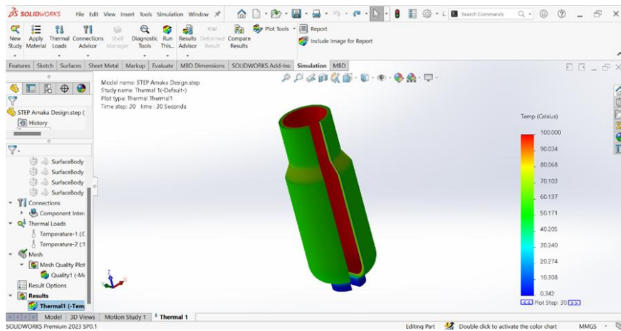
Figure 7: Heat response after some time (30s) of GFRP thermos flask
