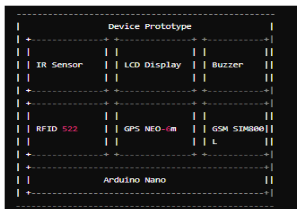
Figure 10: Device Prototype
