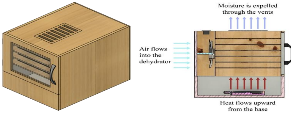
Figure 3: Final model & illustration of the drying process
