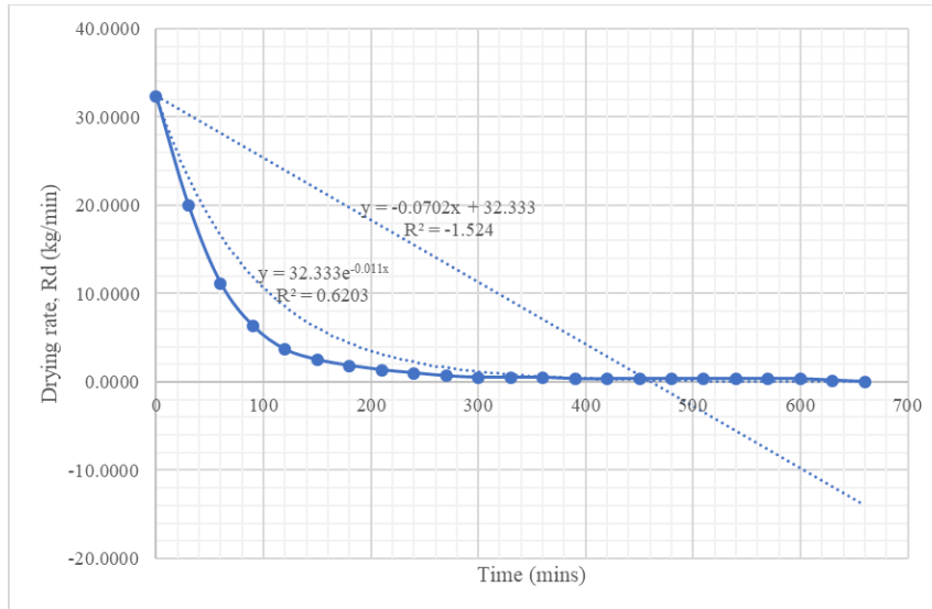
Figure 8: Linear and exponential curve fitting for drying of carrots
