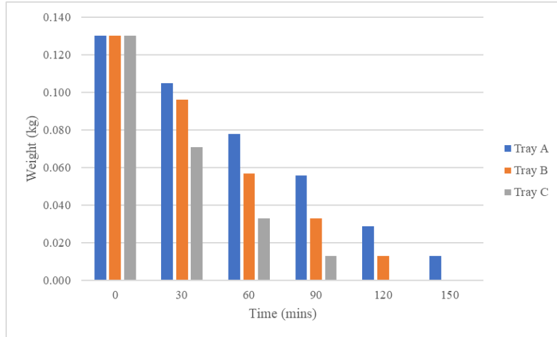
Figure 7: Impact of Tray Position on Drying Time
