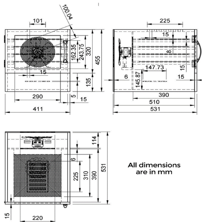
Figure 4: Orthographic views of the model with dimensions
