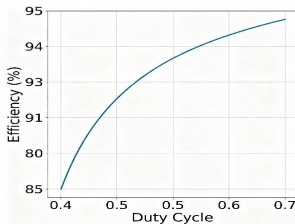
Figure 13: Curve shows duty cycle vs efficiency of DC-DC converter
