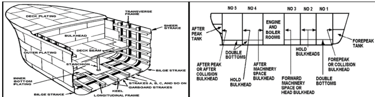
Ship structure
