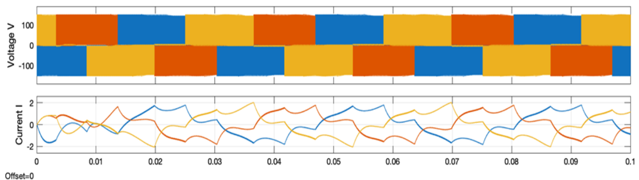
Figure 11: Three-phase inverter output
