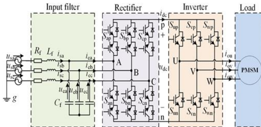
Figure 2: IMC-PMSM topology
