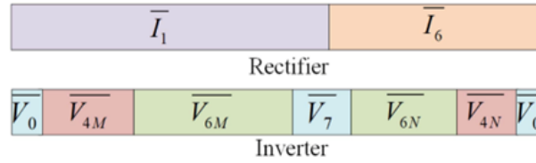
Figure 3: Vector distribution
