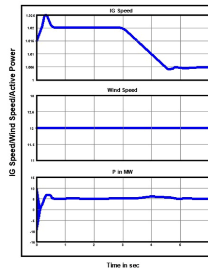
Figure 14: Rated wind speed 12 m/sec w.r. t. time in X axis [22]
