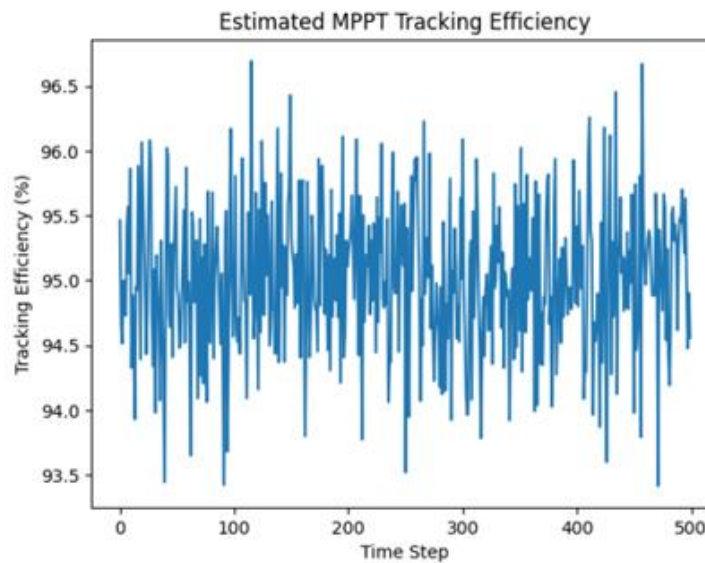
Figure 6: Estimated MPPT tracking efficiency
