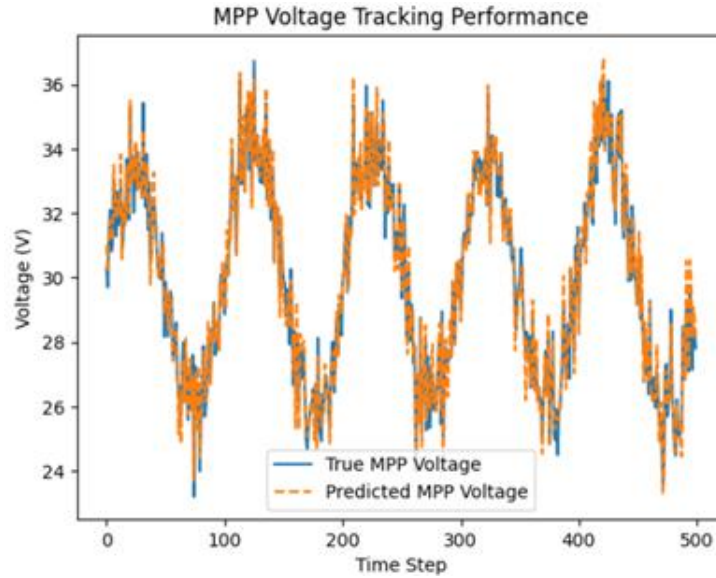
Figure 3: True versus predicted MPP voltage
