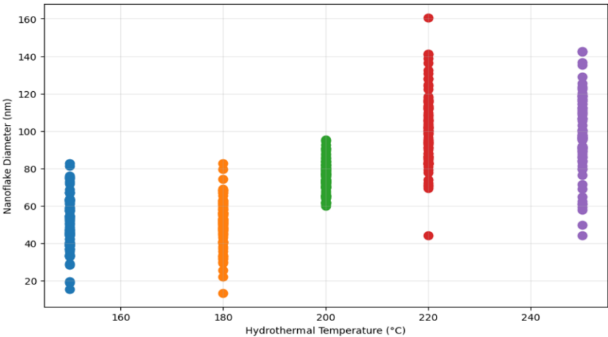
Figure 2: Distribution of nanoflakes diameter and temperature variants
