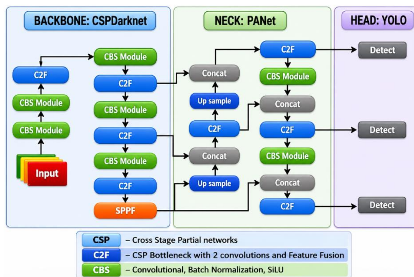
Figure 2: YOLO v8 architecture
