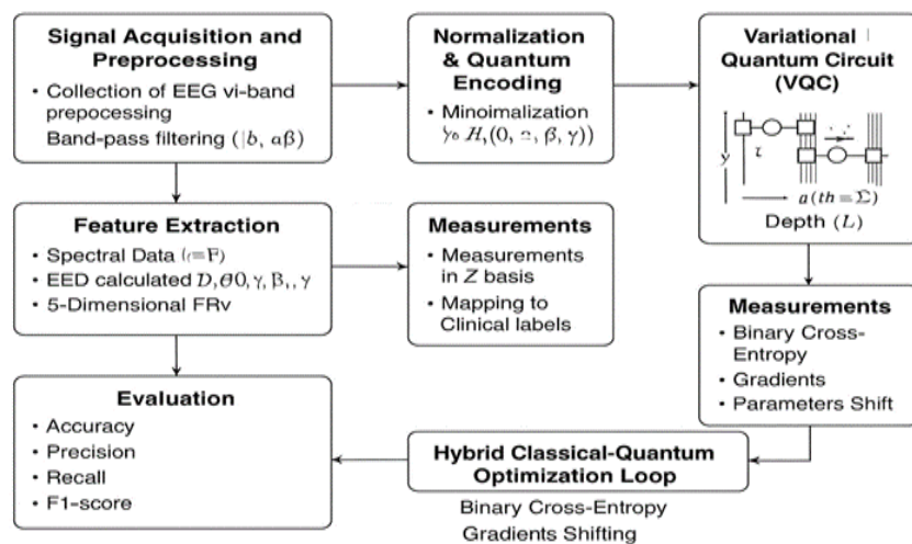
Figure 2: Block diagram
