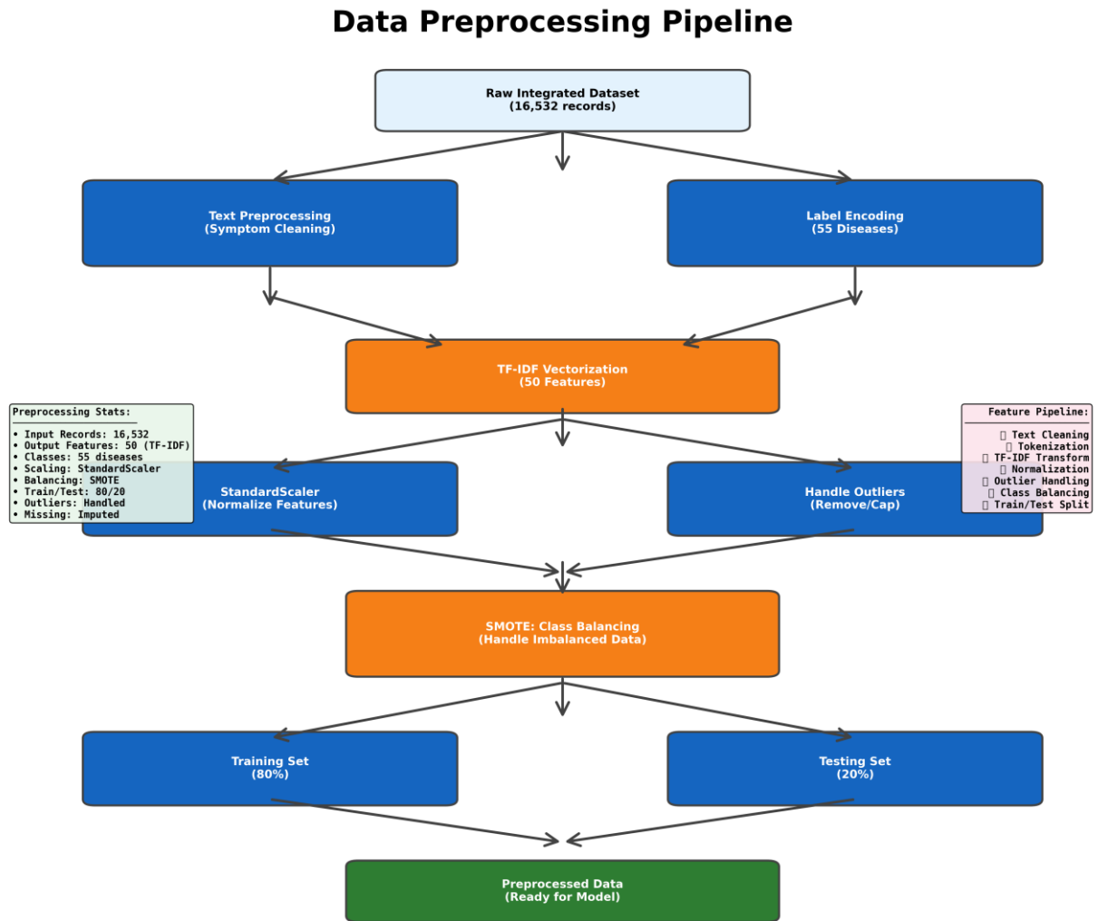
Figure 2: Data preprocessing
