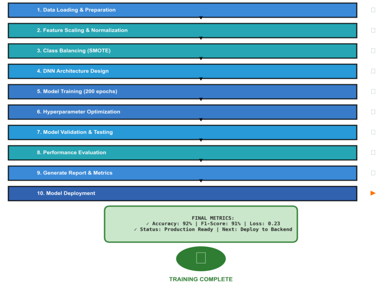
Figure 4: Training pipeline
