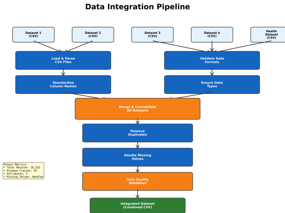
Figure 3: Data integration
