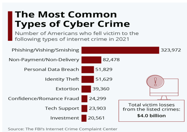
Figure 2: Cyber Attacks [17]
